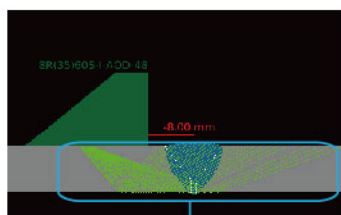
PA beam coverage simulation
